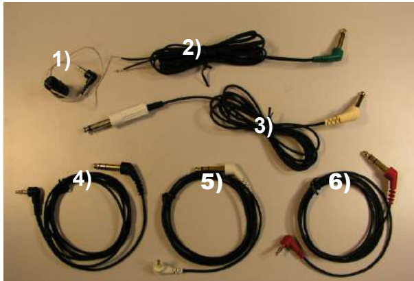
Figure 1: Cable kit
