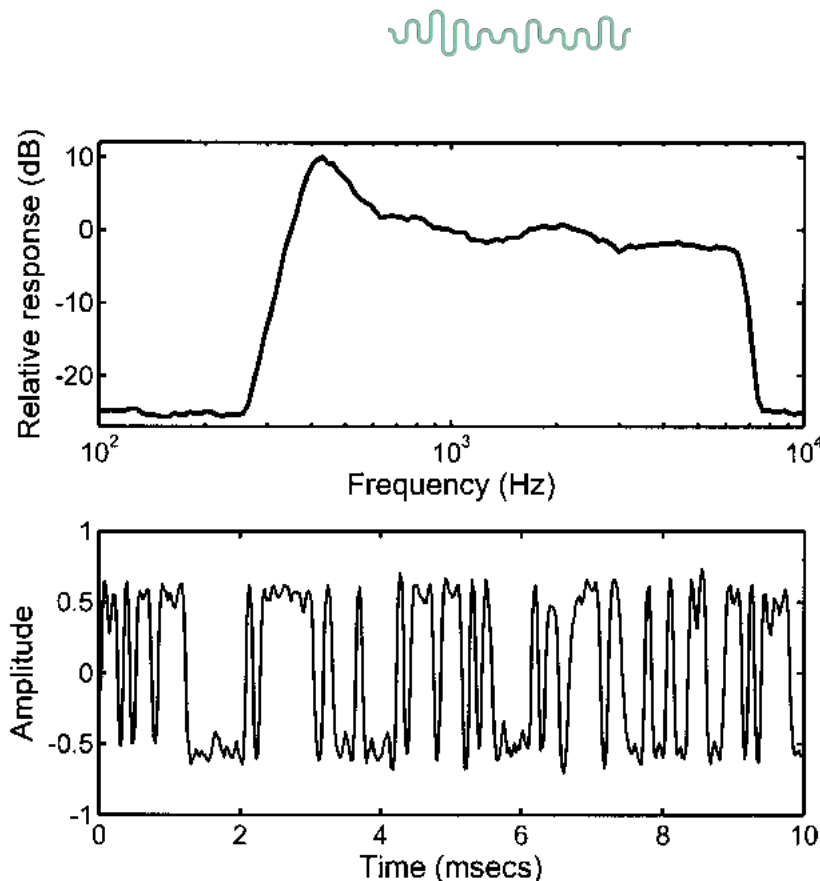
Figure 3: Spectrum (top) and a segment of the waveform (bottom) of the noise used for the TEN(HL) test.
