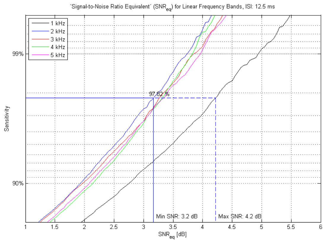
Figure 4: The graph shows the algorithmic sensitivity per frequency band as a function of the SNR_{eq} per band with custom bands (500-1500, 1500-2500, 2500-3500, 3500-4500, 4500-5500). The click repetition interval is 12.5 ms. The graph indicates that the SNR_{eq} increases for low repetition time intervals (faster repetition rates) as long as the test runs for 2 minutes
